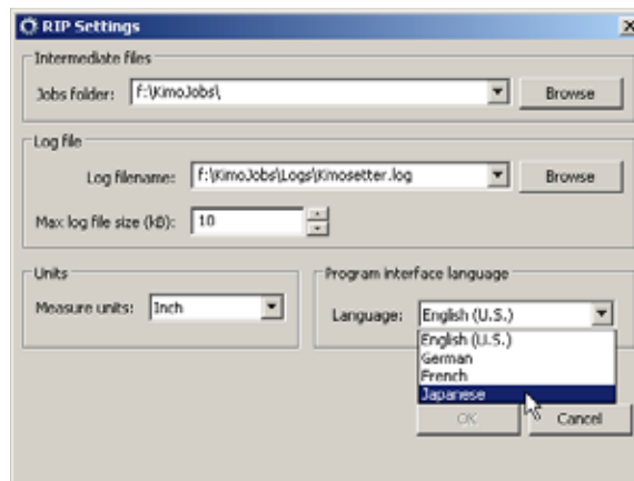
RIP Settings
