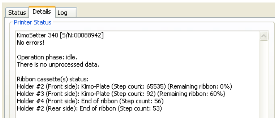
Details tab
